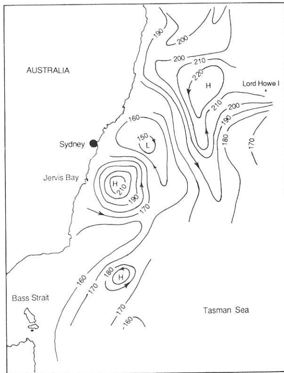
Figure 2. Map of sea surface height off east Australia in January–February 1964. Measurements of the water density at various depths were made at many stations positioned in a grid over the sea. The heights were calculated from the densities. Arrows show direction of currents. The currents are stronger where the lines are closer together. The map shows an eddy off Jervis Bay, and the suggestion of another off Bass Strait. As often found, the East Australian Current is not particularly clear. (Adapted from Deep-Sea Research , vol. 12, 1965, p. 905).
