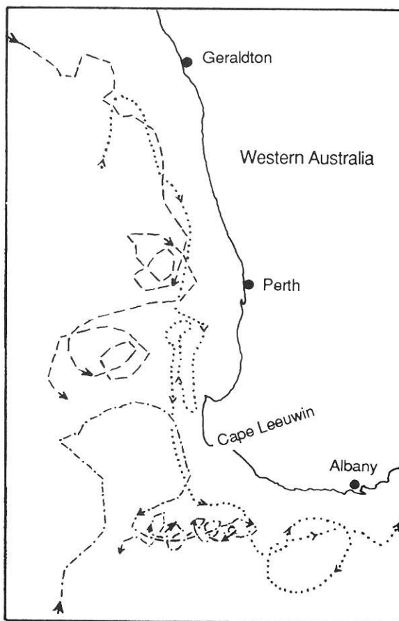
Figure 4. Ocean currents are often studied by releasing drifting buoys, which are tracked by satellite. This figure shows the tracks of three buoys off south-west Australia in March–June 1976. The tendency for the buoys to get trapped in eddies can be seen clearly, especially south-west of Perth. The southward movements near the shelf edge, which is approximately 50 km offshore, are due to the Leeuwin Current. (Adapted from CSIRO Marine Laboratories Research Report 1979–1981).
